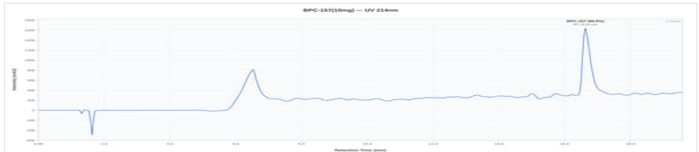
BPC-157 10mg - 1: UV Chromatogram
